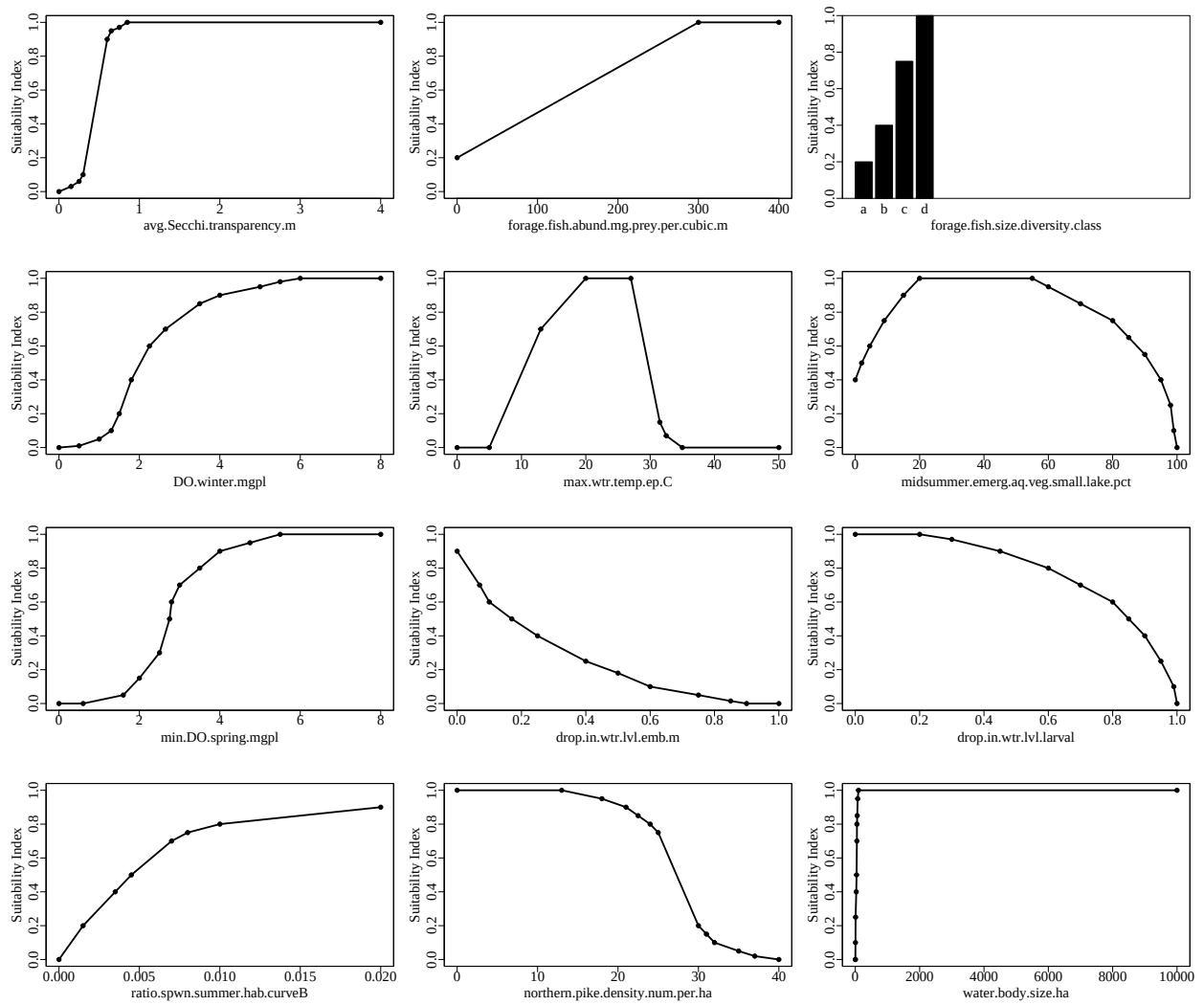
Figure 1. Suitability index graphs for variables included in the muskellungeSmallLakeSpwnVegCurveB model in ecoest.
